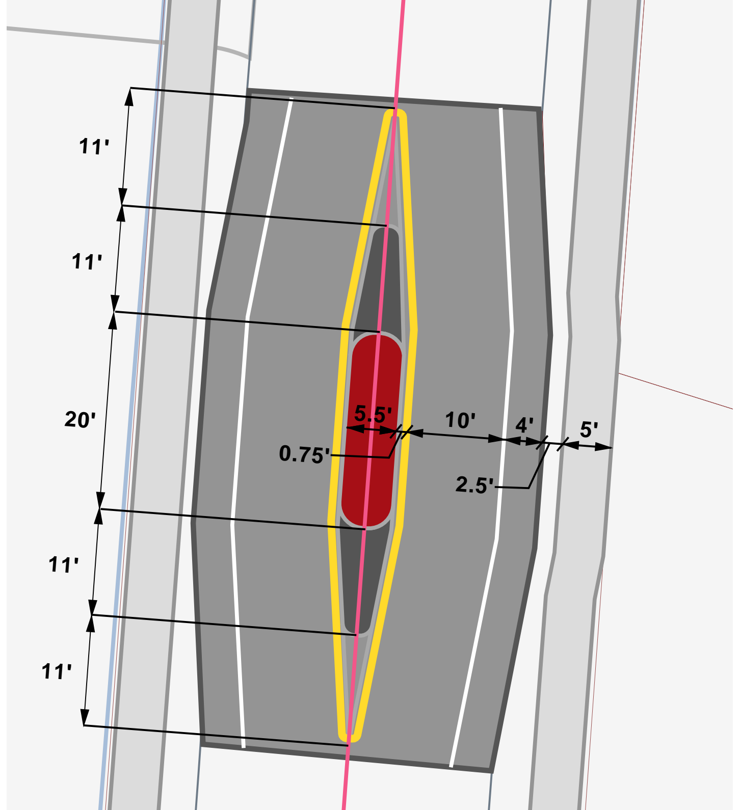
Median Island Detail
