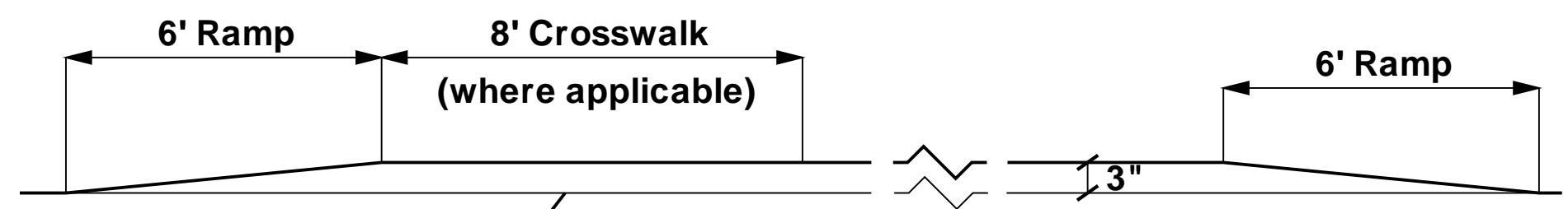
Raised Intersection Profile
