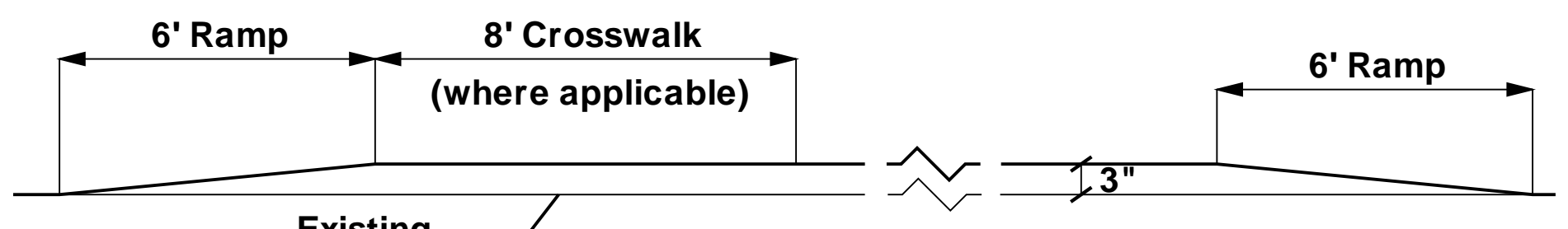
Raised Intersection Profile
