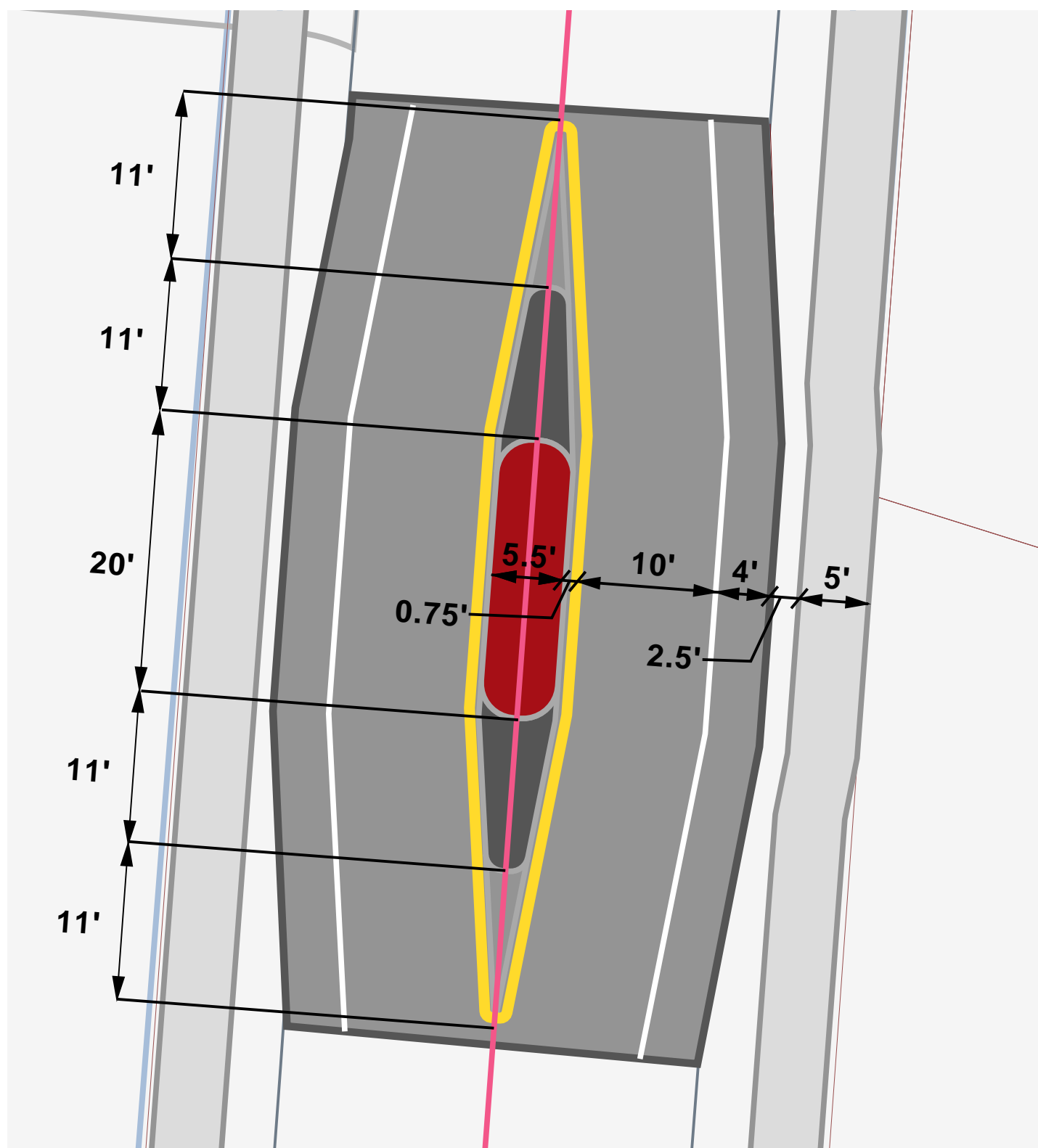
Median Island Detail
