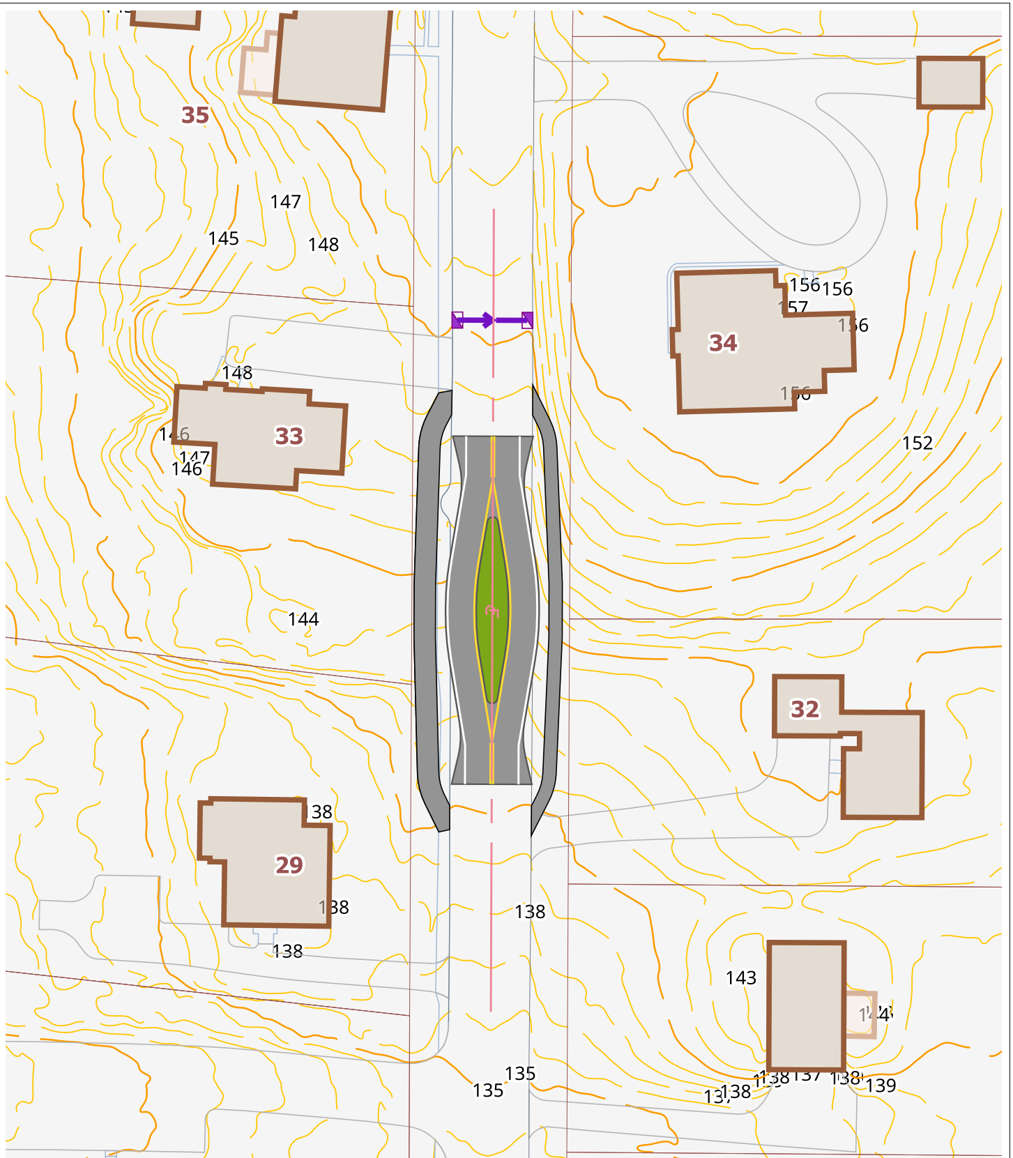
Bloomfield Traffic Calming - Woodland Avenue 1000' North of Wintonbury Avenue Offset Choker Scale 1"=60' W-1
