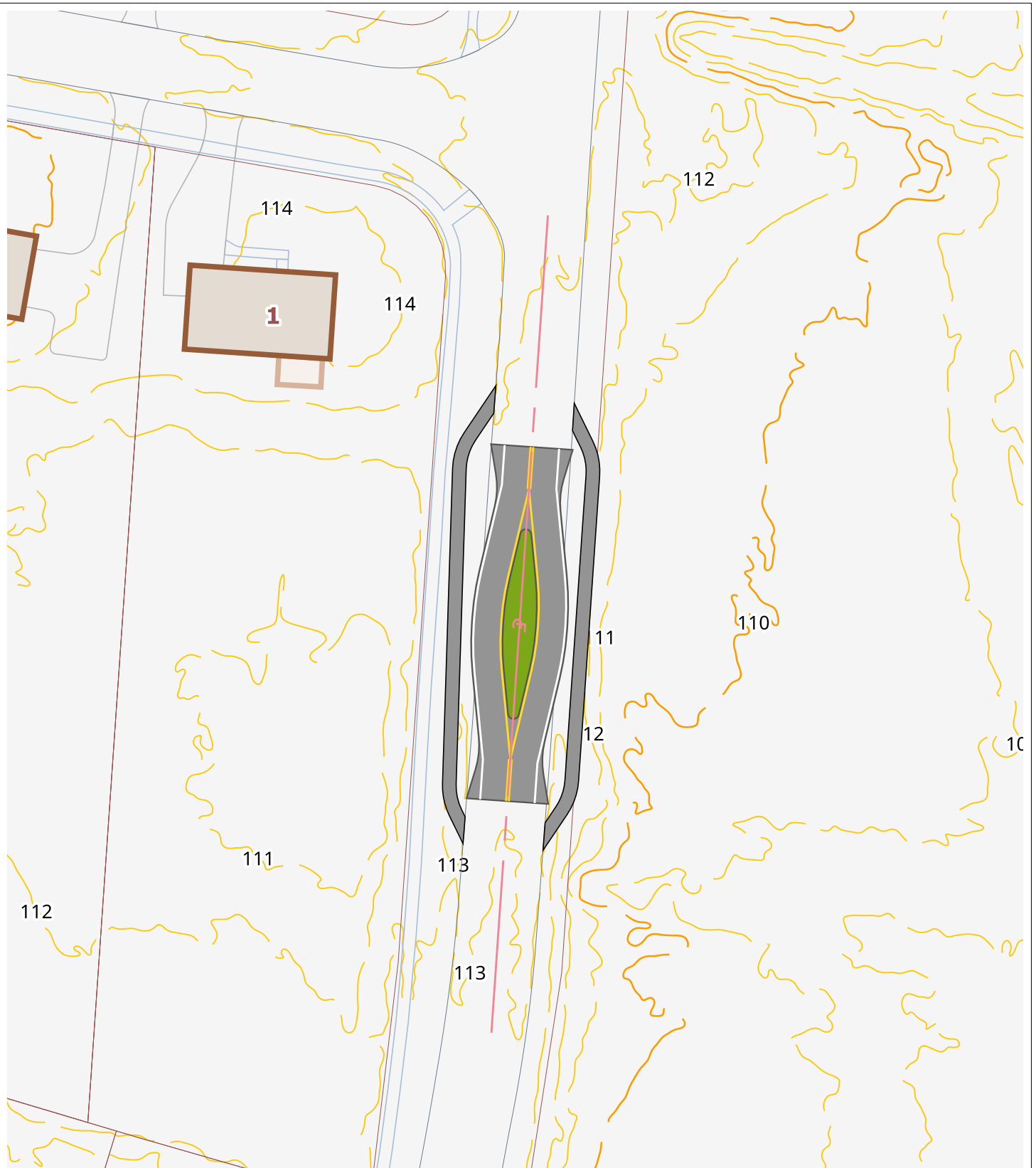
Bloomfield Traffic Calming - Woodland Avenue 100' South of Evan Lane Offset Choker Scale 1"=60' W-5
