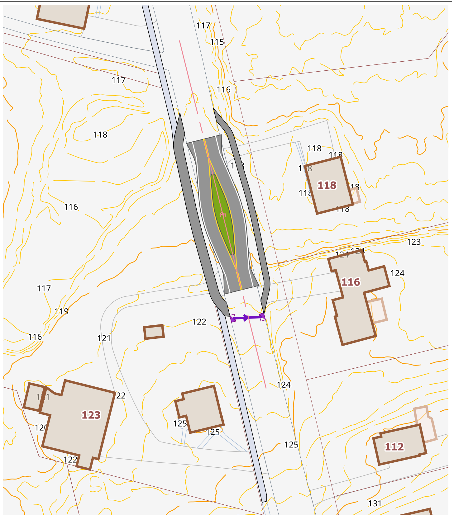
Bloomfield Traffic Calming - Woodland Avenue 600' South of Ashley Court Offset Choker Scale 1"=60' W-4
