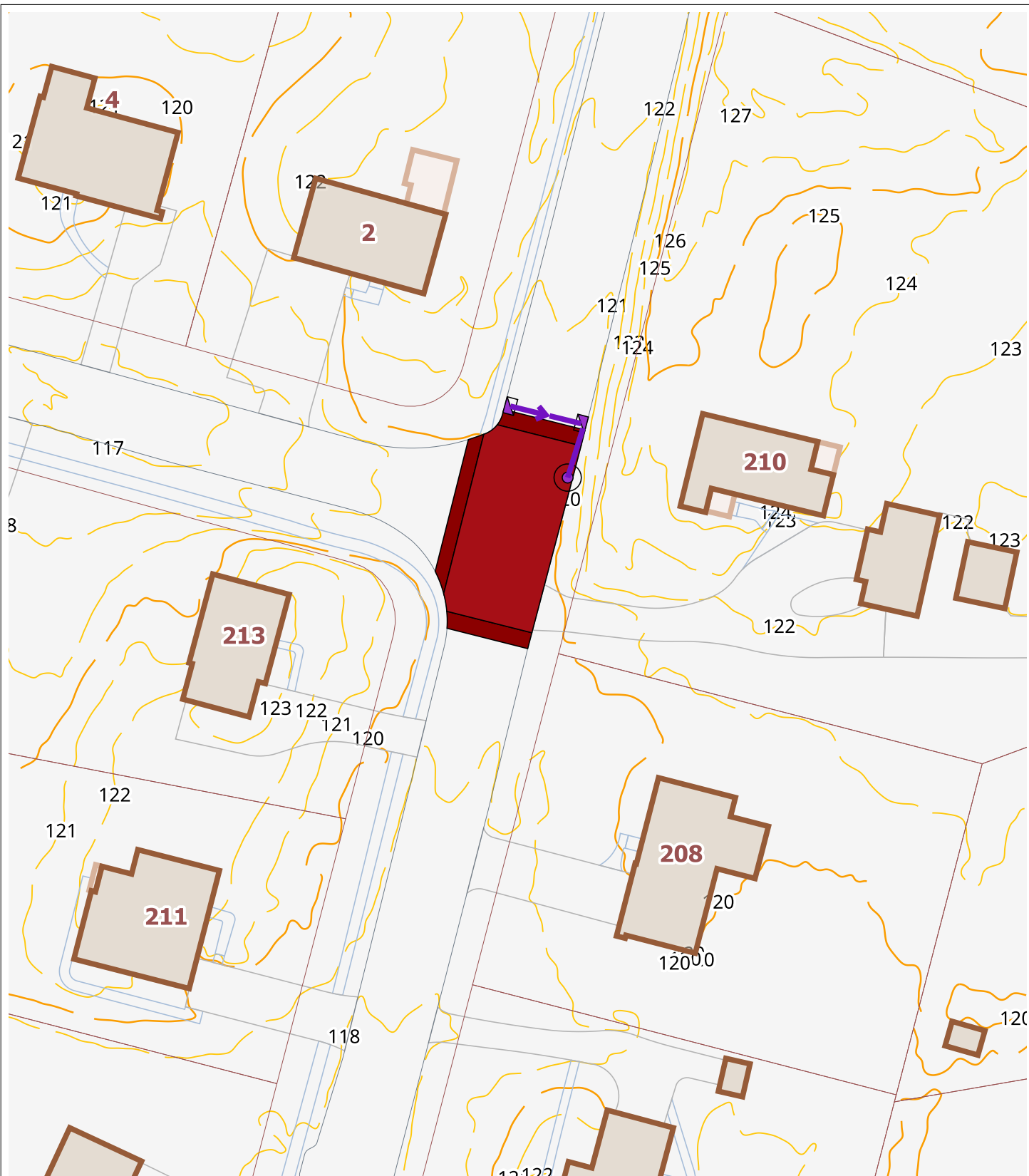
Bloomfield Traffic Calming - Woodland Avenue At Linwood Drive Raised Intersection Scale 1"=60' W-7
