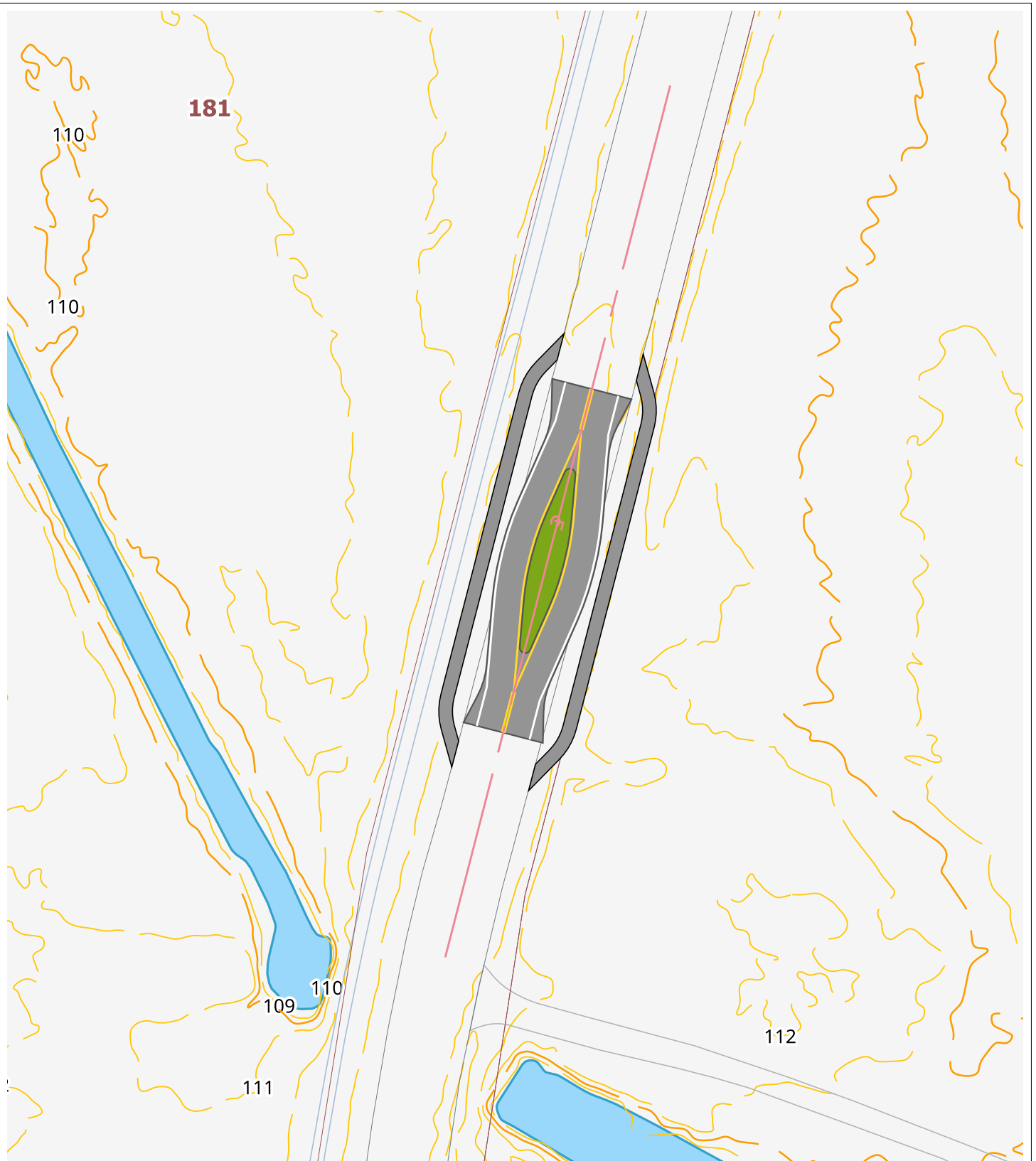
Bloomfield Traffic Calming - Woodland Avenue 600' North of Evan Lane Offset Choker Scale 1"=60' W-6
