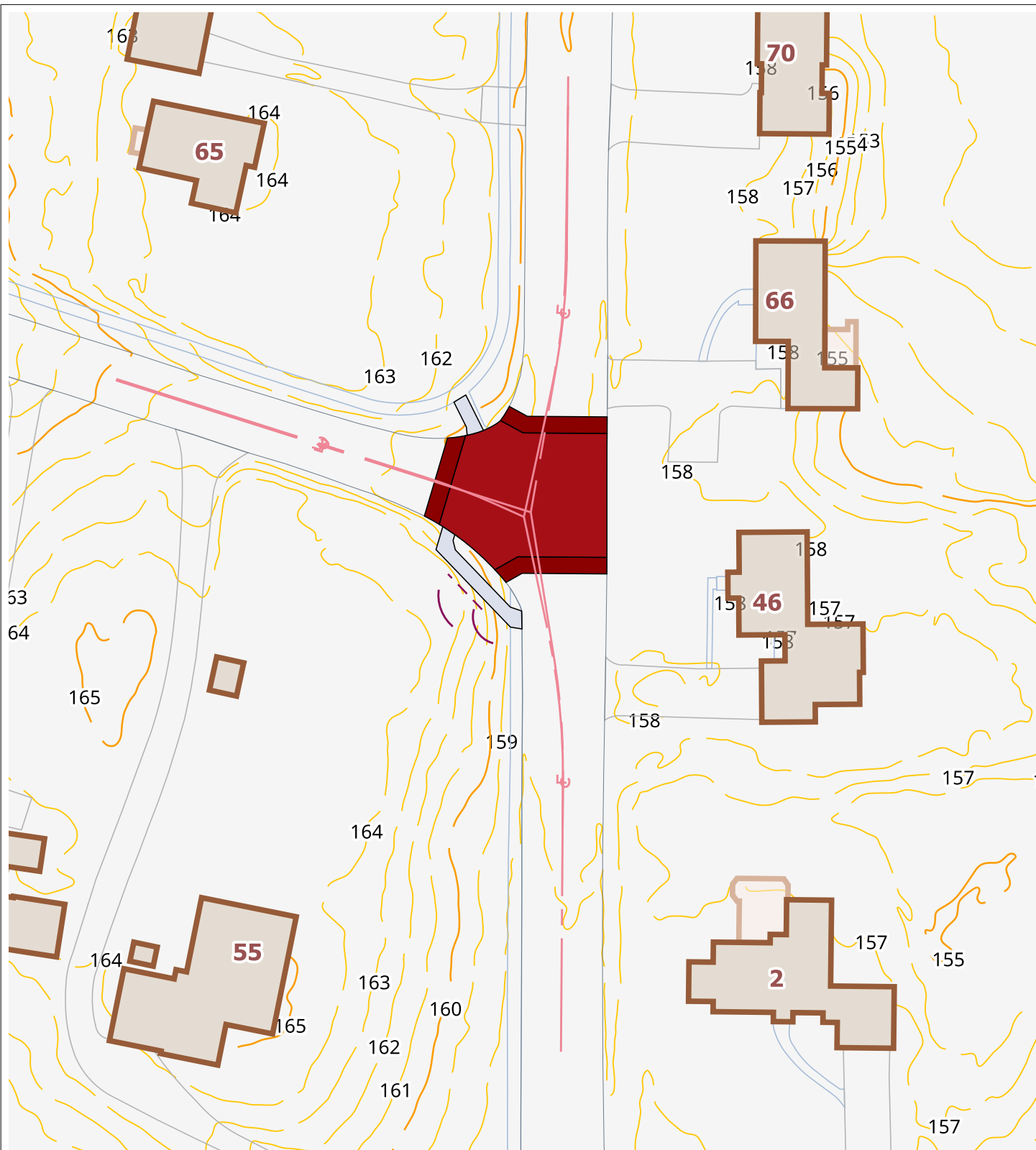
Bloomfield Traffic Calming - Woodland Avenue At Mills Lane Raised Intersection Scale 1"=60' W-2
