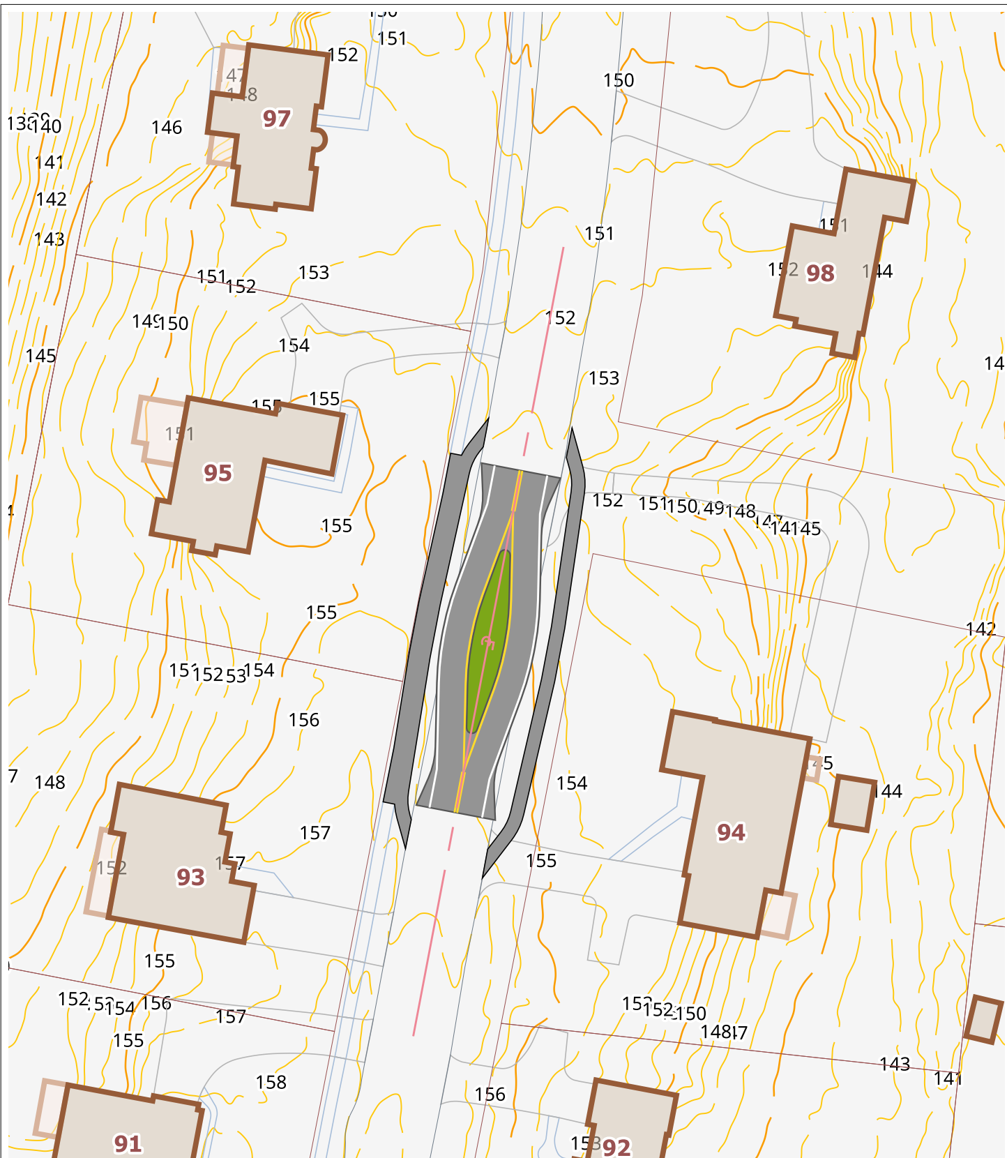
Bloomfield Traffic Calming - Woodland Avenue 800' North of Mills Lane Offset Choker Scale 1"=60' W-3
