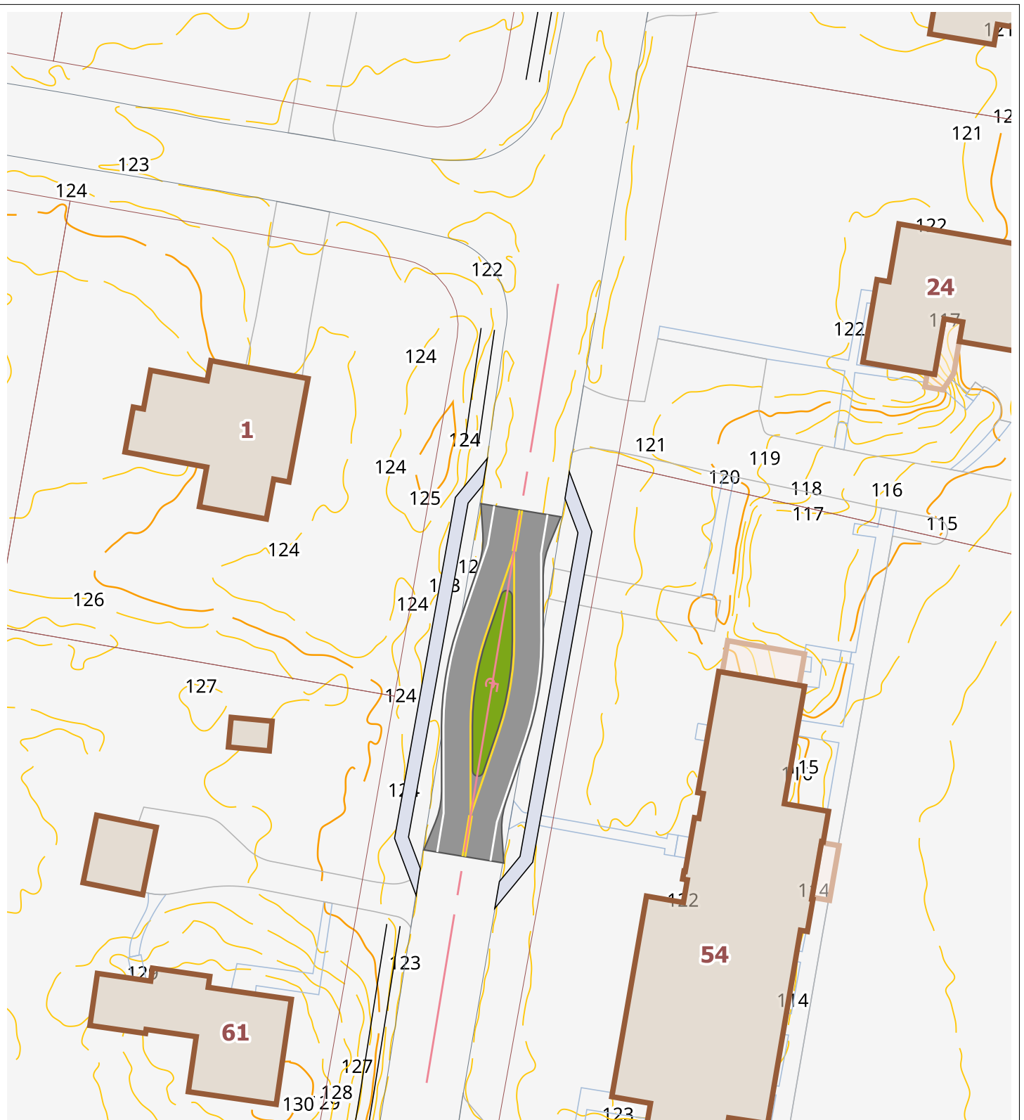
Bloomfield Traffic Calming - Maple Avenue 300' South of Mallard Drive Offset Choker Scale 1"=60' M-3
