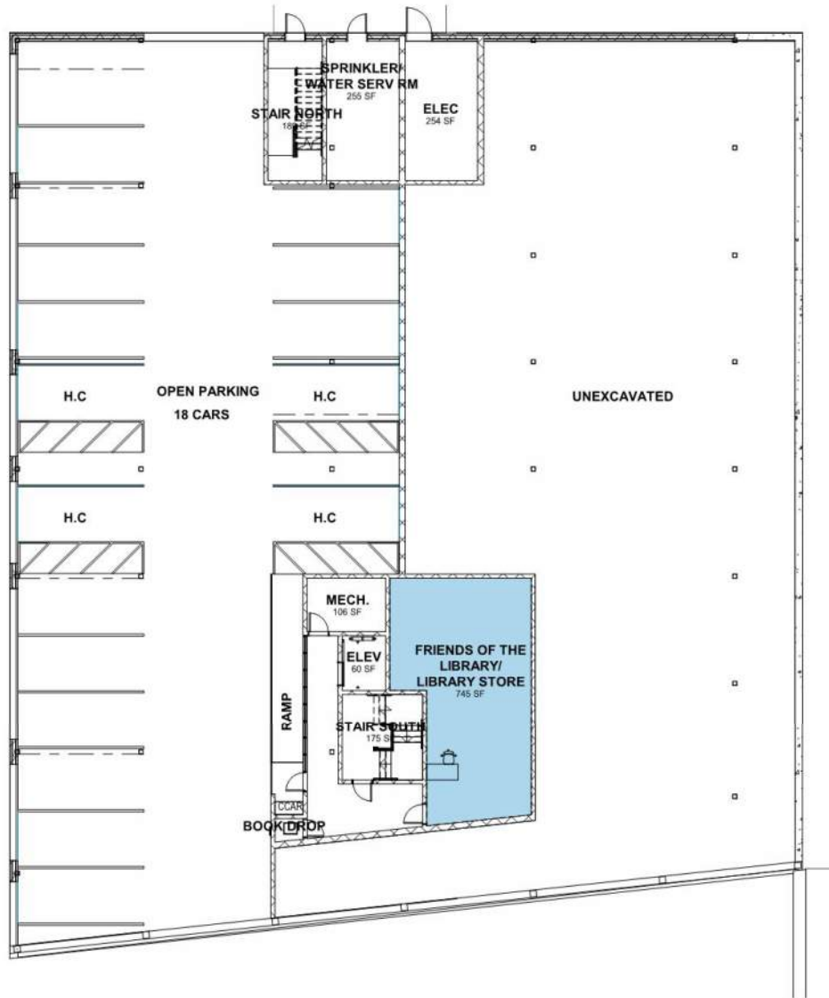
1 LOWER LEVEL PLAN AREAS 1/16" = 1'-0"
