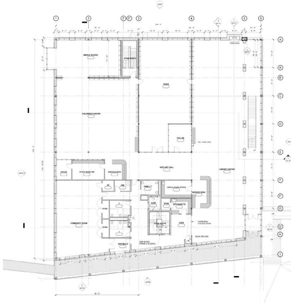
1 FIRST FLOOR PLAN 1/8" = 1'-0"
